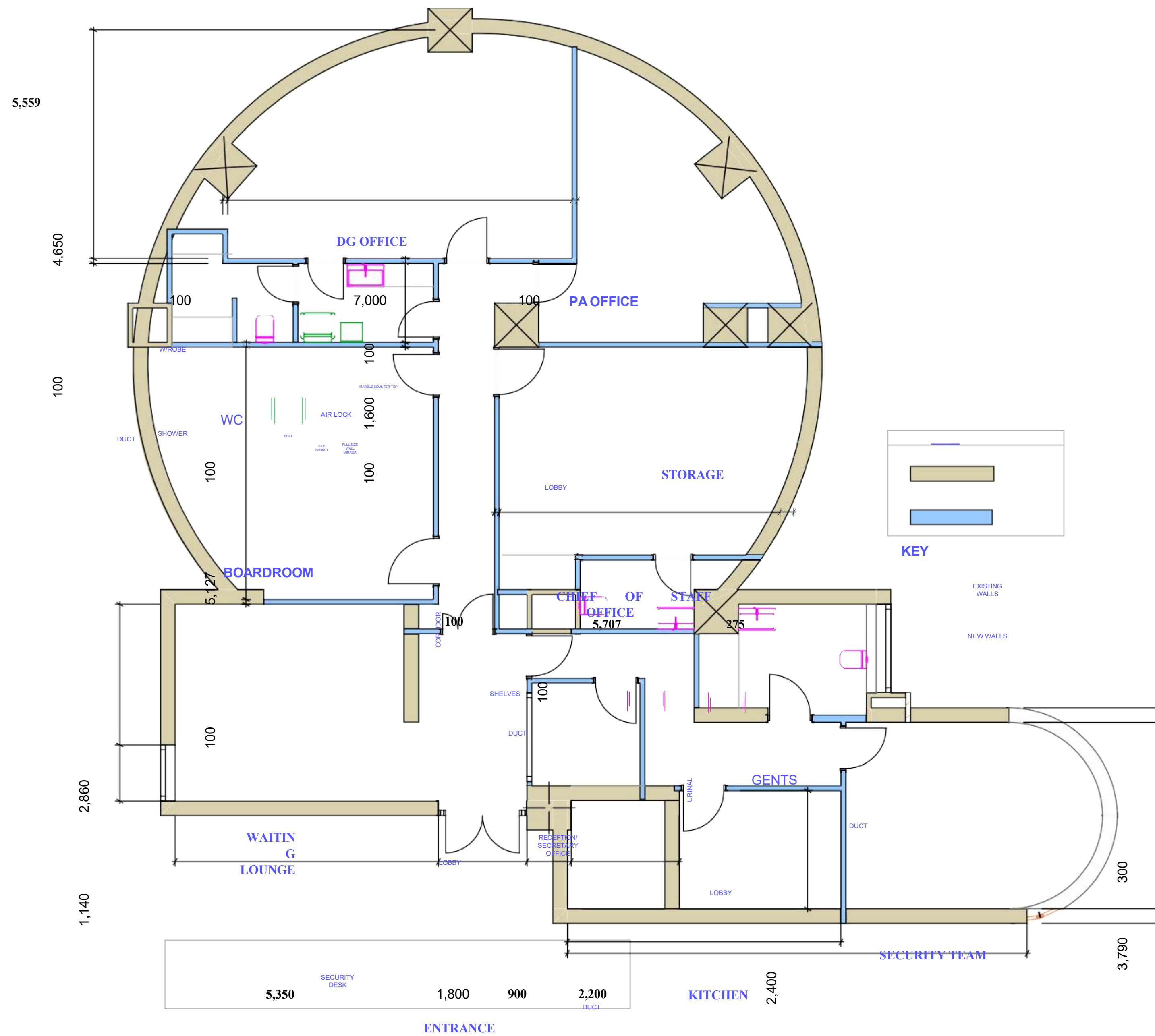
PROPOSED COAST GUARD OFFICES ON 12TH FLOOR BAHARI TOWER
